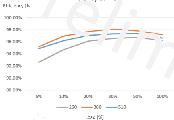
Efficiency Curve
